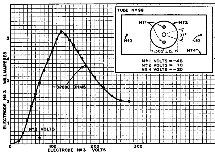
Fig. 17—Negative impedance by change of focus.
